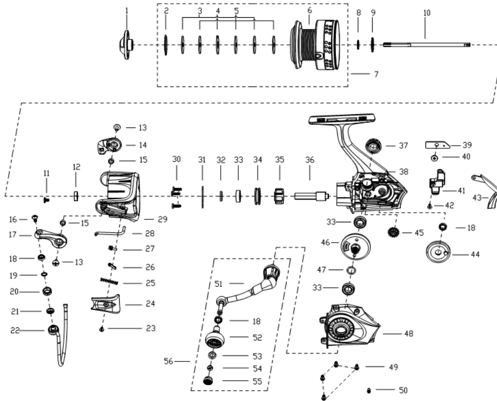
PARTS LIST OF MAXPROSP 60
